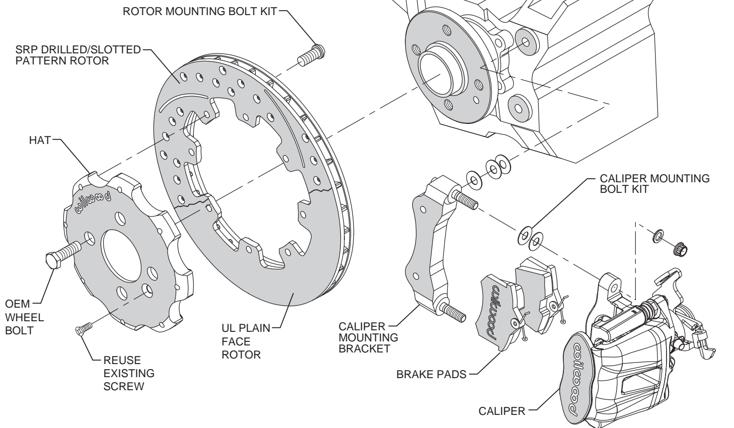
Typical Installation Diagram, Major Components Identified.
